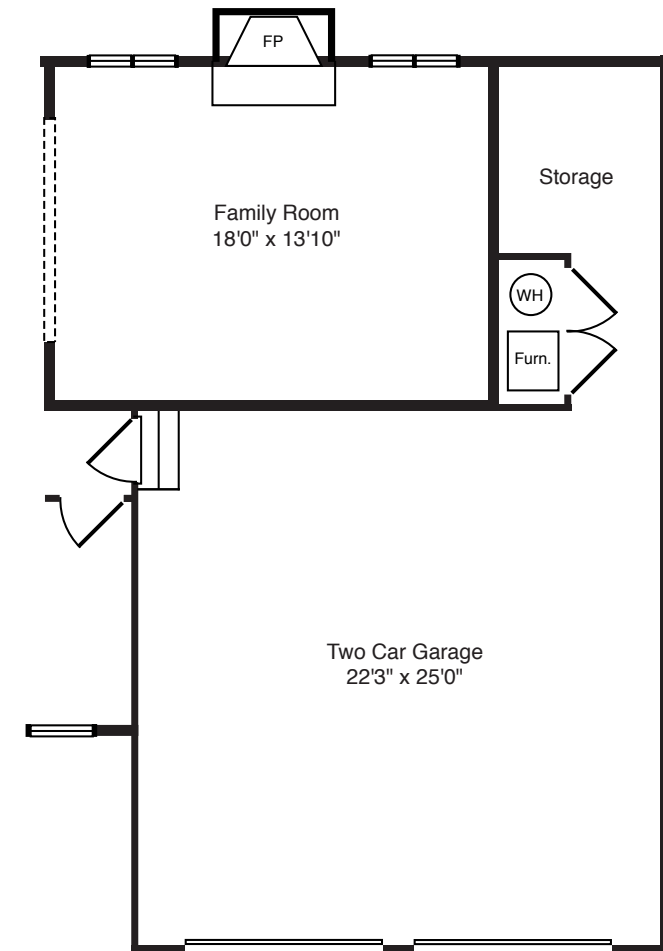
2280 Garage Storage w/Slab Option
